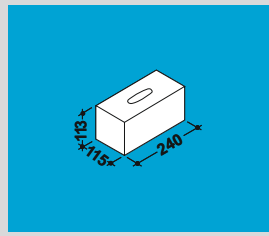
KS-2DF 240/115/113 mm
